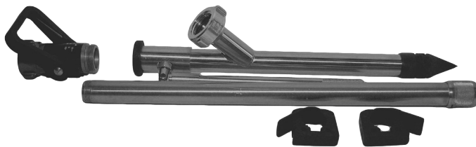
902 - without shutoff valve 902K - with shutoff valve
